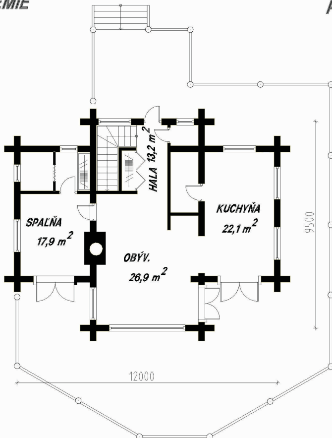
PRIZEMIE
